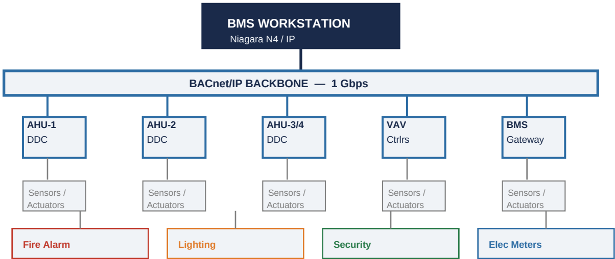
Figure 3 — BMS Network Architecture (Schematic — Not to Scale)
